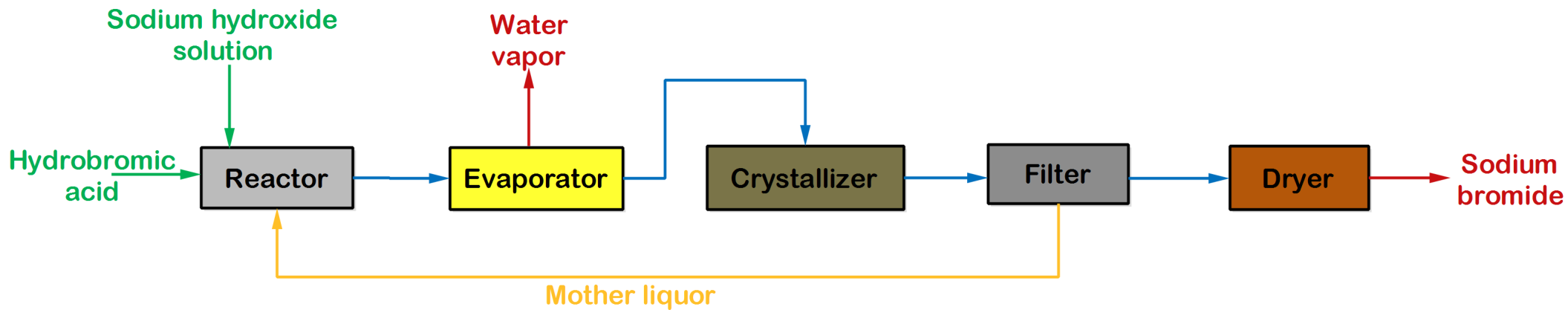
Figure: Manufacture of sodium bromide by neutralization
